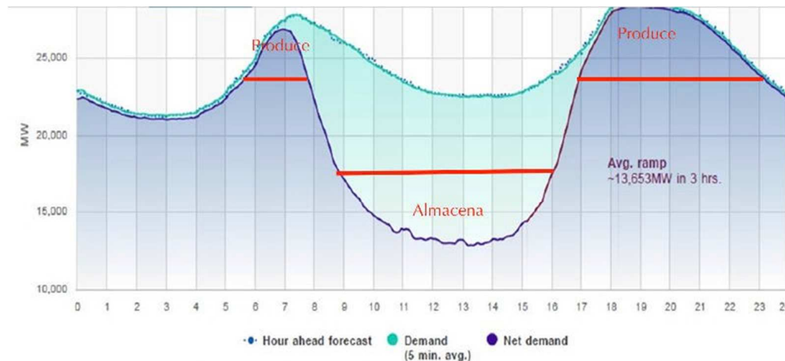
The Duck: CAISO Total Demand and Net (of Solar and Wind) Demand for Feb 7, 2019 (source: http://www.caiso.com/Today%20Outlook/Pages/default.aspx )
